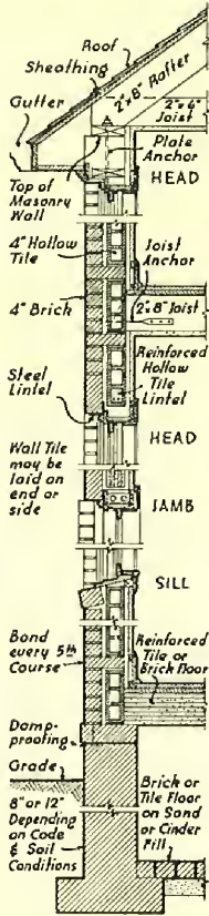
Wall Section
